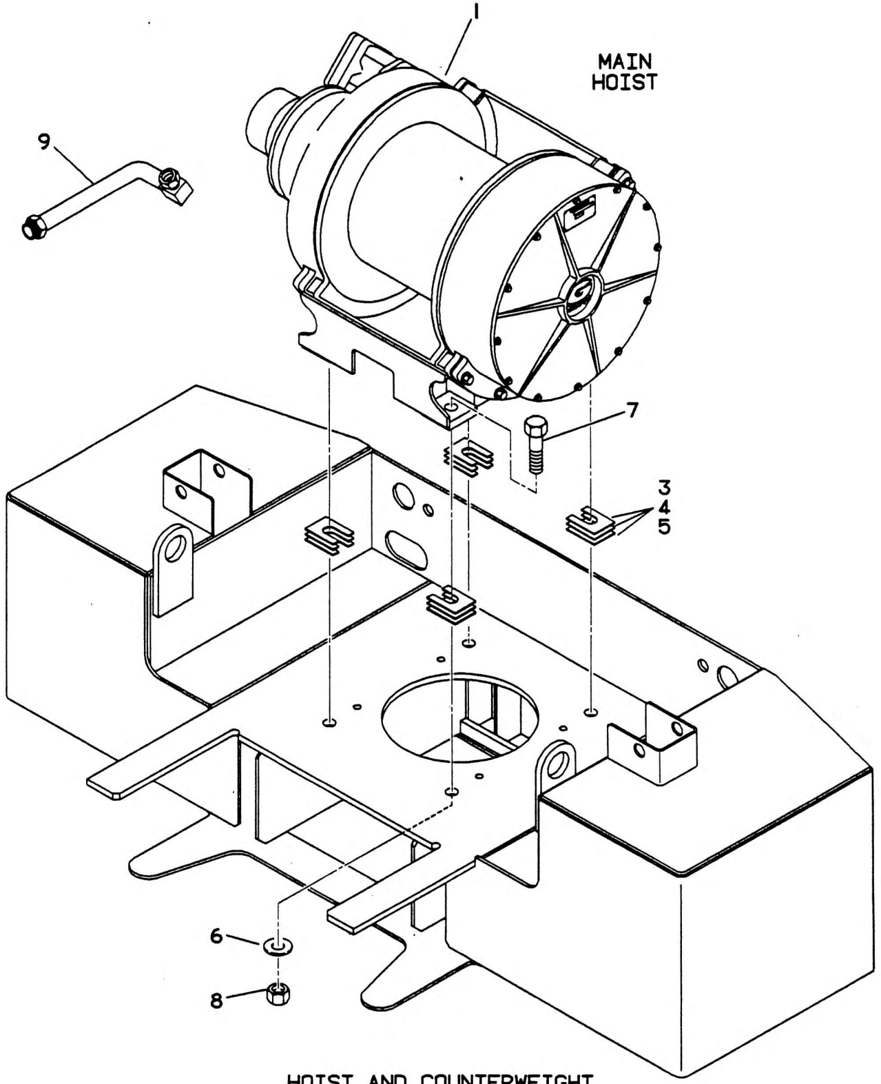
HOIST AND COUNTERWEIGHT MOUNTING WELDMENT.
